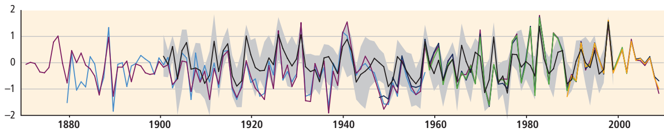
(c) The December to March Pacific North American (PNA) pattern
