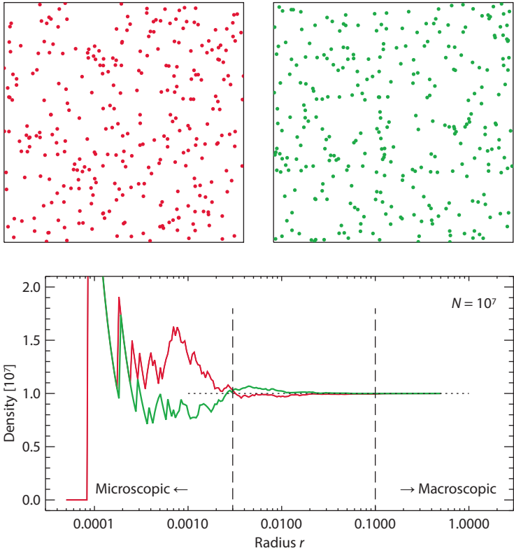
Figure 1.1. Going from the microscopic to the macroscopic scale. The top panels show two distinct random distributions of N = 300 particles in the unit square. The bottom panel shows the result of using equation (1.1) to calculate the particle density, based on a series of circles of increasing radii, concentric and centered on the middle of the unit square, now for two distinct random distributions of N = 10^7 particles. Note the logarithmic horizontal axis. The resulting density curves differ completely for radii smaller than a few times the mean interparticle distance \delta = 0.0003 , but converge to the expected value of 10^7 particles per unit area for radii much larger than this distance (see text).
