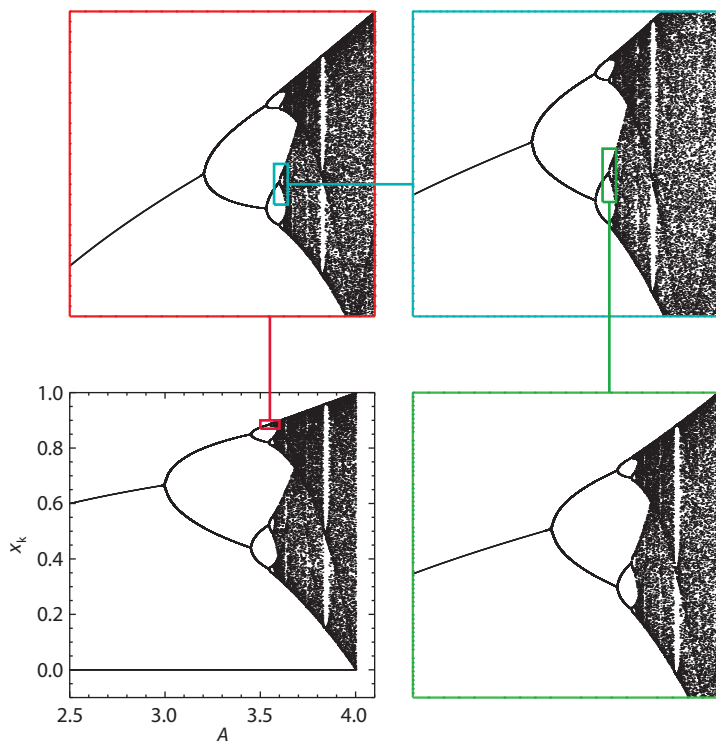
Figure 1.2. Bifurcation diagram for the logistic map (bottom left), as given by equation (1.2). The first bifurcation from the trivial solution x_n = 0 occurs at A = 1.0 , off to the left on the horizontal scale. The other three frames show successive nested close-ups (red→blue→green) on the period-doubling cascade to chaos.
